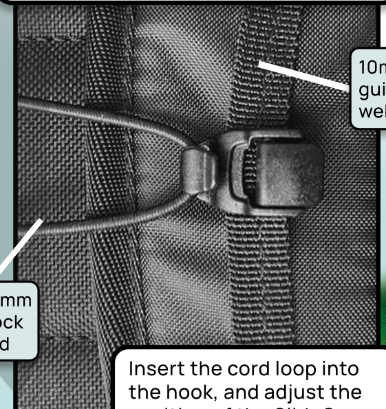
SlideCam Hook 100-0810
